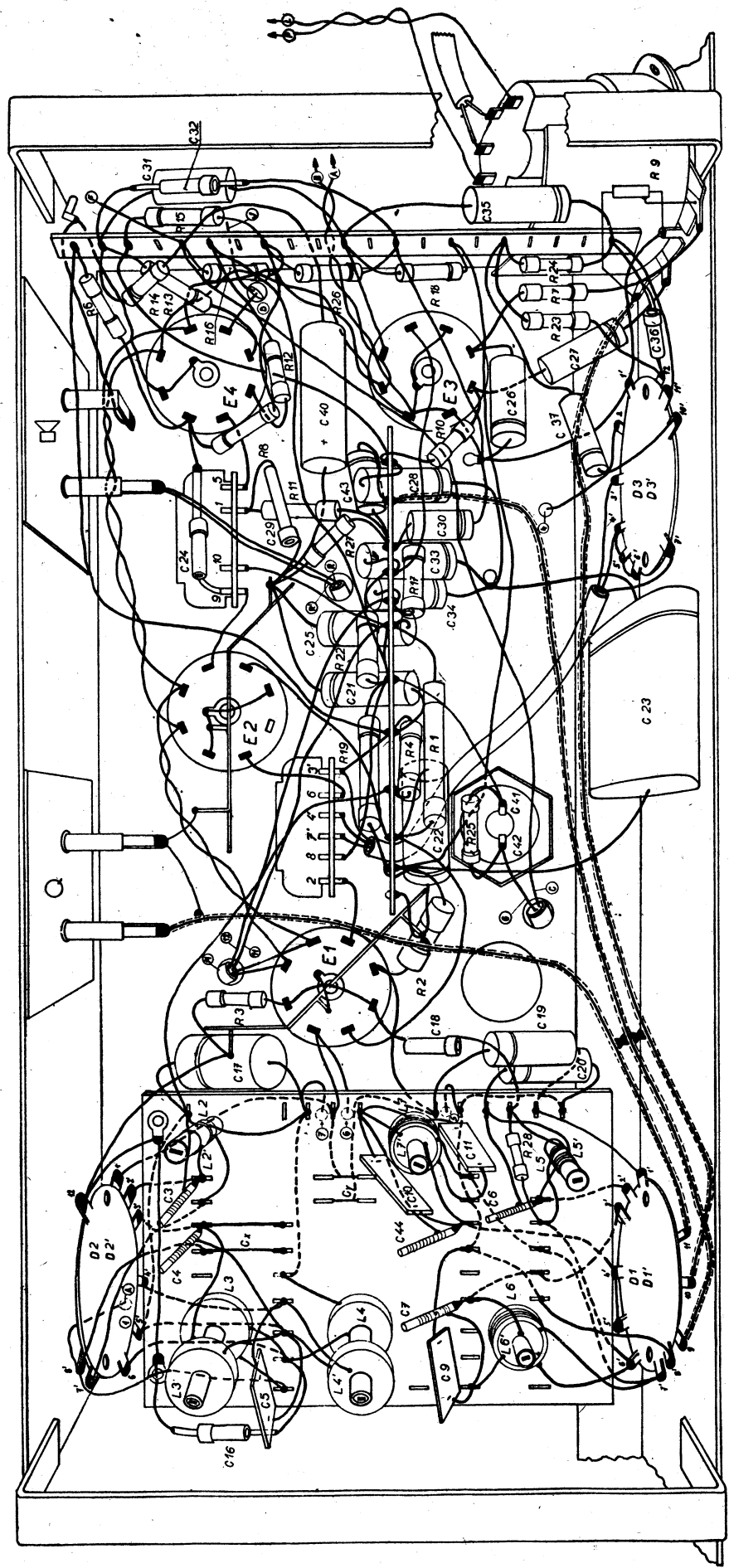
Obr. 8. ZAPOJENI PRIJIMATEL POD CHASSIS
